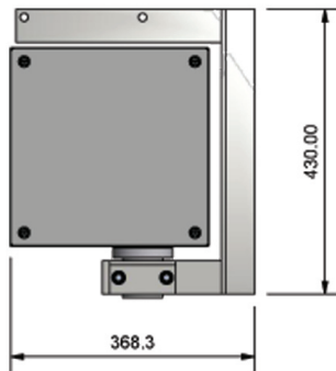
Top Entry Terminal Box with Fixing Bracket
