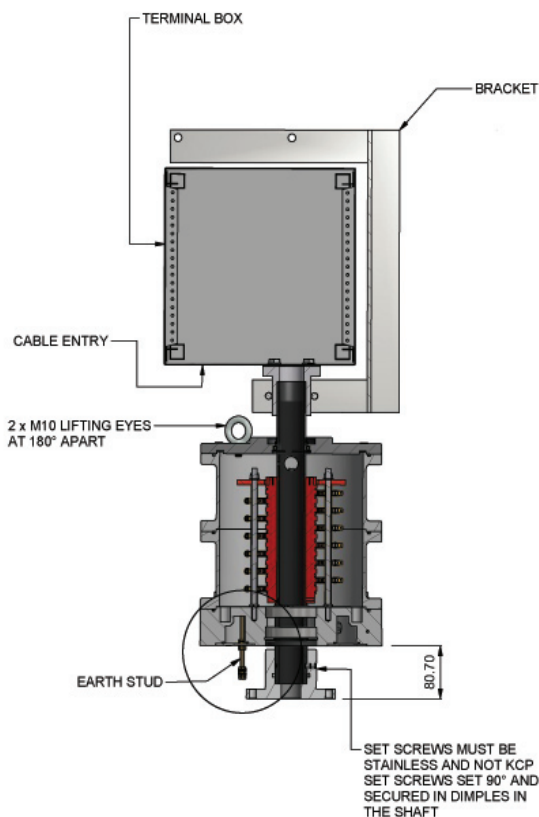
Top Entry Terminal Box Attached to SPB Unit
